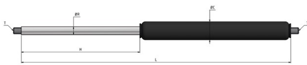
Gas spring – Steel (piston rod: chromium-plated, cylinder: black spray coated)
