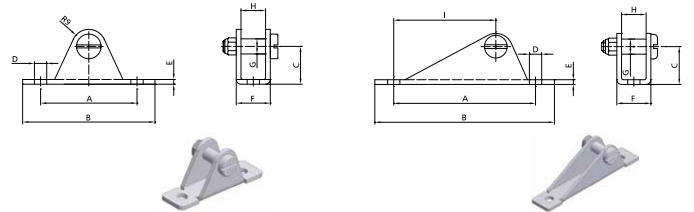
Clevis bracket
